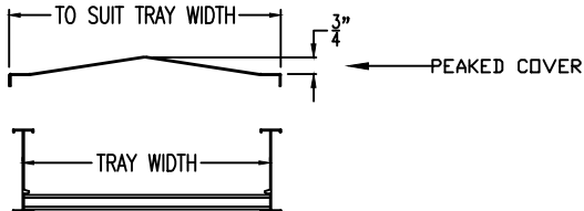
END VIEW
